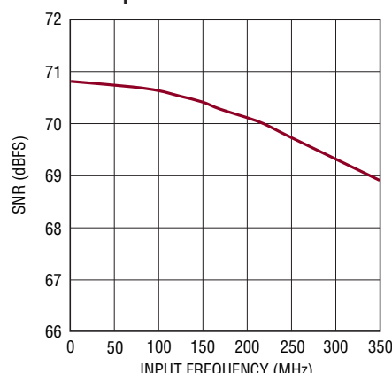
LTC2264-12: SNR vs Input Frequency, -1\text{dBFS} , 2\text{V} Range, 40\text{Mps}
